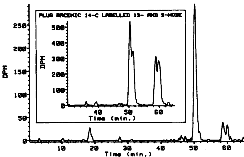
Fig. 7. Representative straight-phase chiral HPLC radiochromatograms of the methyl esters of the radio-labeled 13- ^{14}\text{C} ]HODE and 9- ^{14}\text{C} ]HODE produced in the incubation of ^{14}\text{C} ]linoleic acid with hair roots epilated from the scalp of a normal male. The outer chromatogram is that of the material in the peak at 20.5 min (Fig. 2, upper chromatogram) which was then subjected to the chiral-phase chromatography shown here. The methyl ester of 13-HODE elutes prior to that of 9-HODE and the S -stereoisomer of each compound is the first to elute under these chromatographic conditions. The chromatogram shown in the inset is that of an equal aliquot of the same material to which racemic 13- ^{14}\text{C} ]HODE and 9- ^{14}\text{C} ]HODE methyl ester standards had been added. The mixing experiment demonstrates that the principal product of the incubation of linoleic acid with hair roots is 13( S )-HODE, with racemic 9-HODE constituting a minor product.
